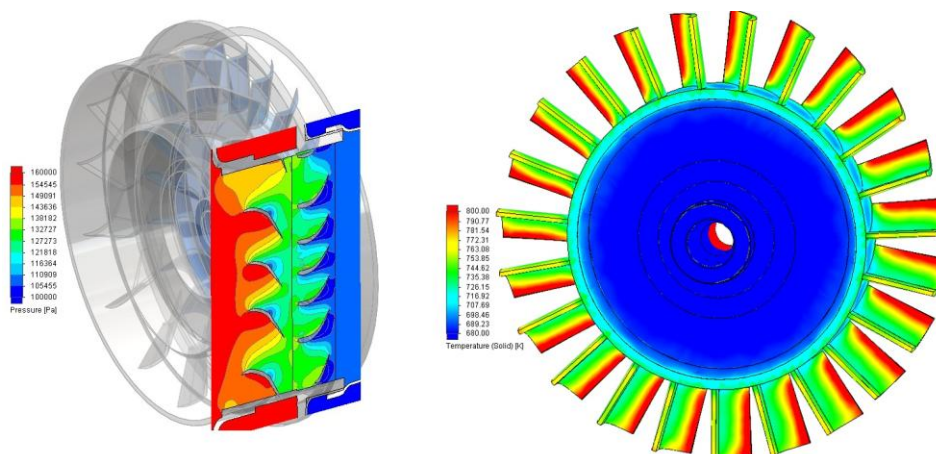
Figure 19. Pressure distribution at a section of the NGV and the turbine (left) and temperature distribution on the turbine's blades at the normal mode.
