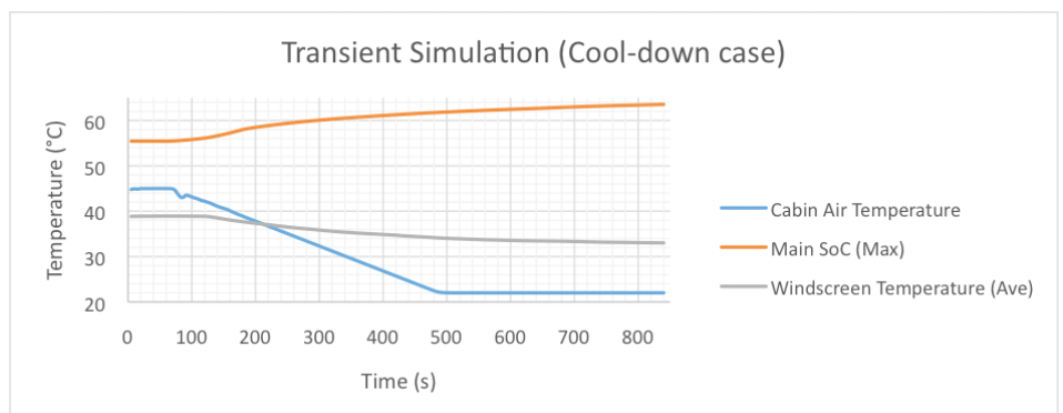
Figure 4. Key temperatures during transient cool-down simulation
