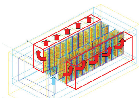
Figure 9. Hot aisle containment within the datacenter
