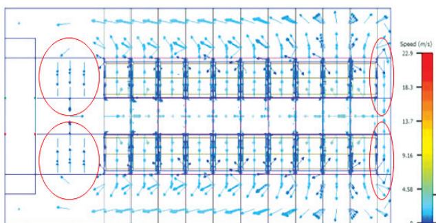
Figure 8. Velocity plot of the simulation results shows the air circulation within the datacenter
